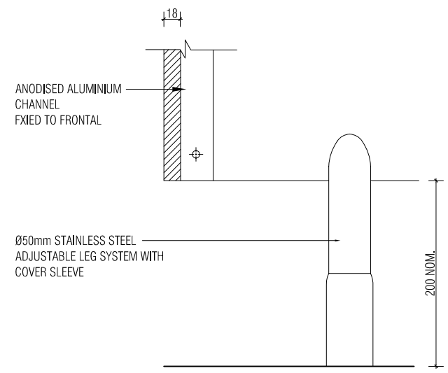
07 FLOOR LEG SECTION 1:2
