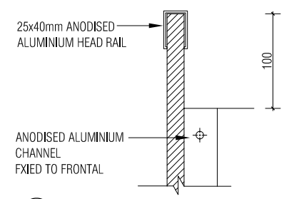
06 HEAD RAIL DETAIL 1:2
