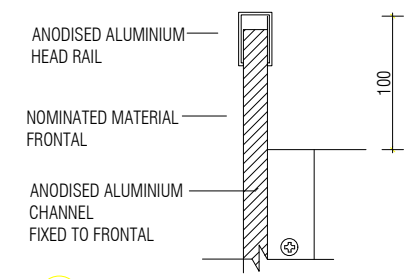
06 HEAD RAIL DETAIL 1:2
