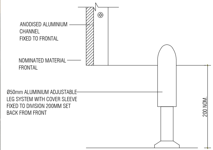
07 FLOOR LEG SECTION 1:2
