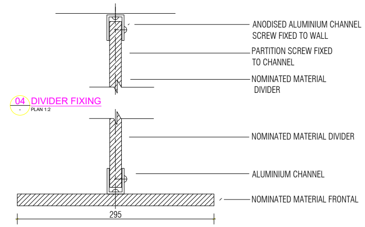
04 DIVIDER FIXING PLAN 1:2
