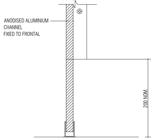
07 FLOOR LEG SECTION 1:2
