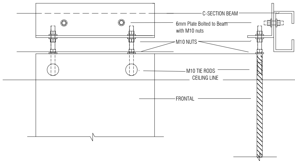
06 FRONTAL FIXING - ELEVATION 1:2
