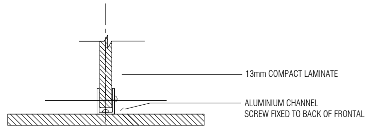
05 FRONTAL FIXING (2G) - PLAN 1:2
