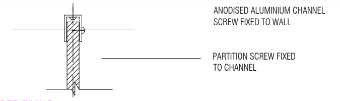
04 DIVIDER FIXING - PLAN 1:2
