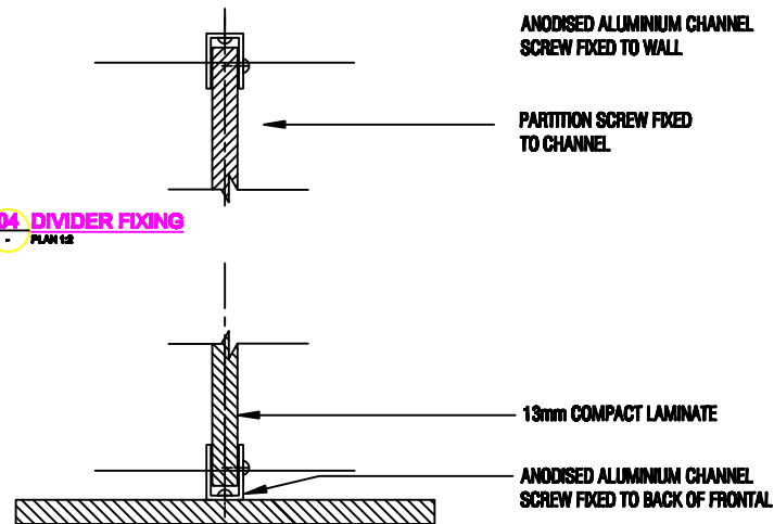
05 FRONTAL FIXING (3G) PLAN 12
