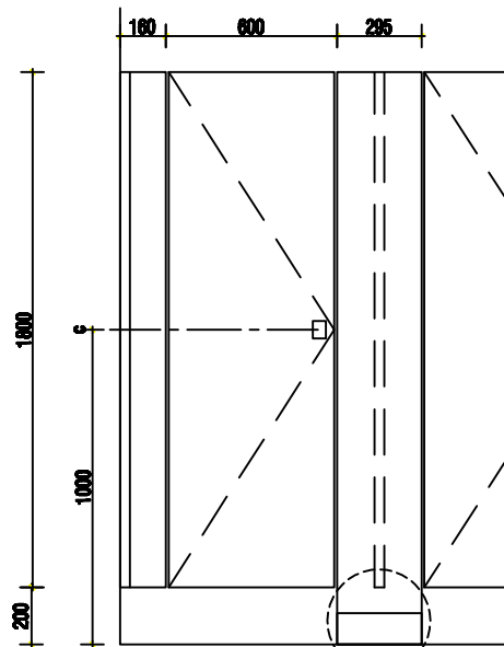
03 ELEVATION
