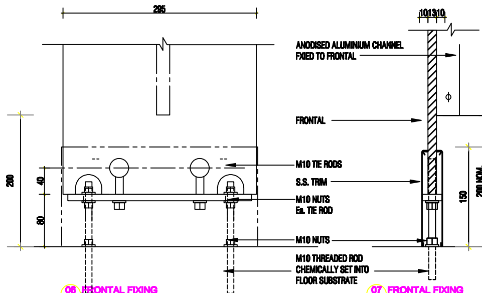
06 FRONTAL FIXING ELEVATION 12
