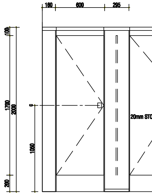
03 ELEVATION SCALE 1:10
