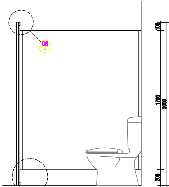
02 ELEVATION SCALE 1:10
