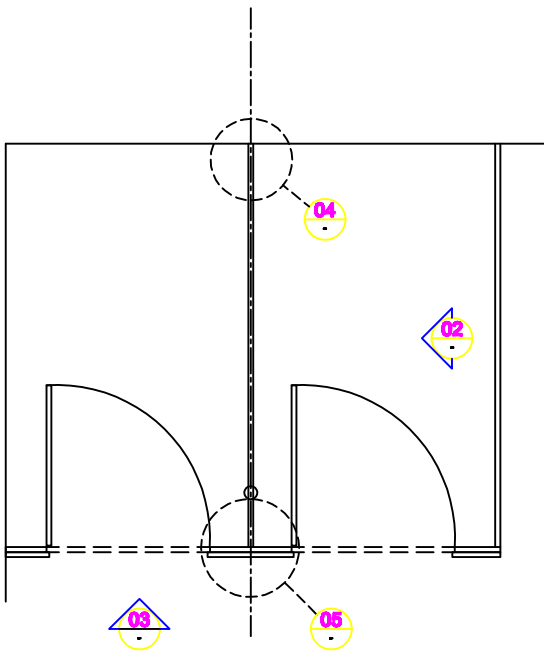
01 PLAN SCALE 1:10
