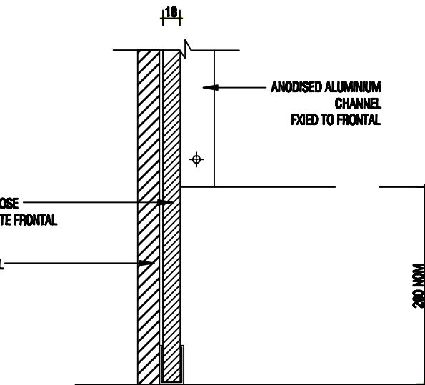
07 FLOOR LEG SECTION 1:2
